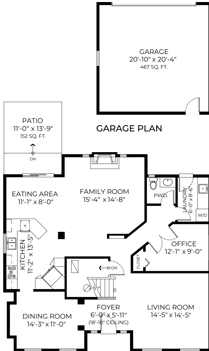
MAIN FLOOR PLAN Ceiling Height: 9'-0"
