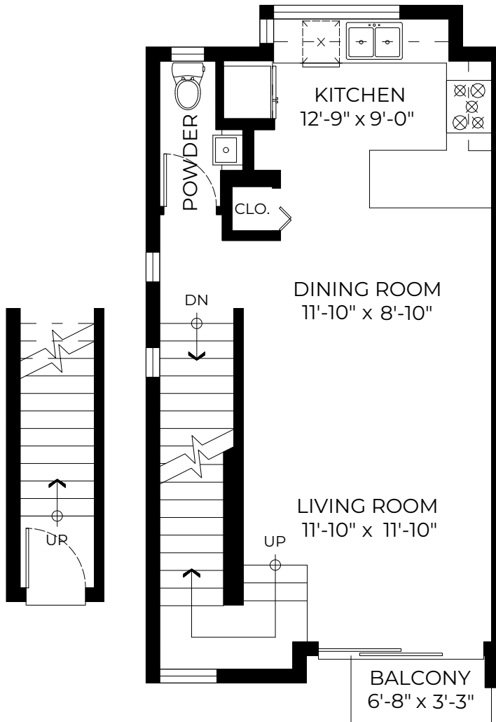
MAIN FLOOR PLAN Ceiling Height: 9'-0"
