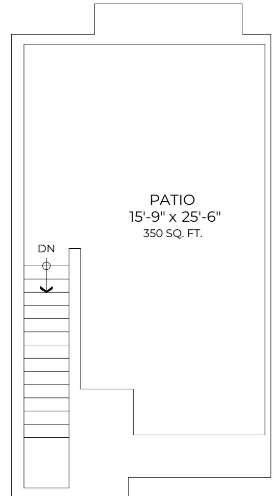
ROOFTOP PLAN
