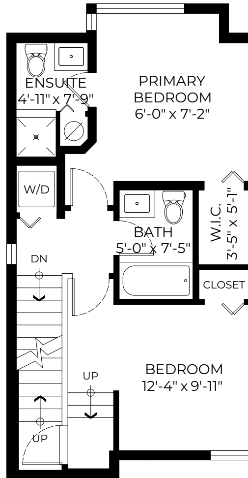
UPPER FLOOR PLAN Ceiling Height: 8'-0"
