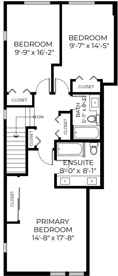
UPPER FLOOR PLAN Ceiling Height: 8'-0"
