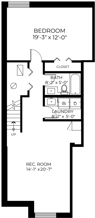
LOWER FLOOR PLAN Ceiling Height: 8'-0"
