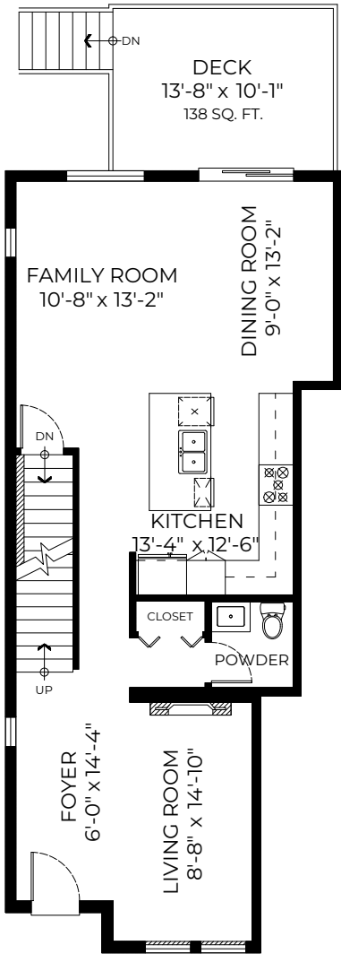
MAIN FLOOR PLAN Ceiling Height: 9'-0"
