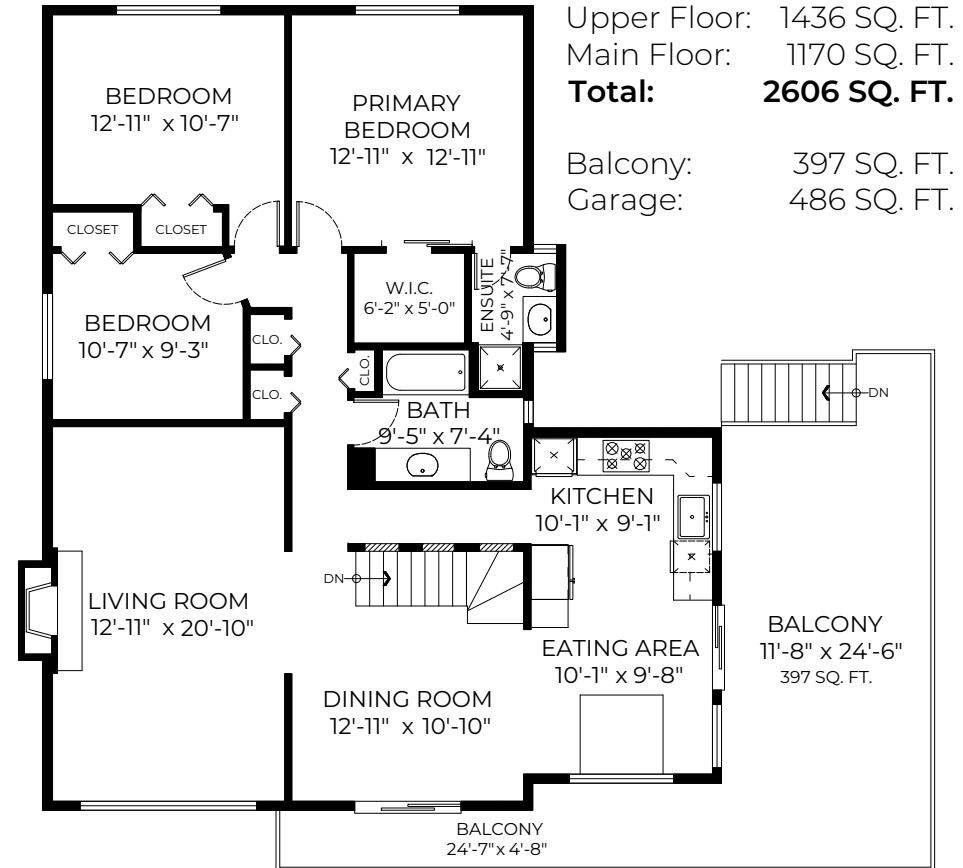
UPPER FLOOR PLAN Ceiling Height: 8'-0"
