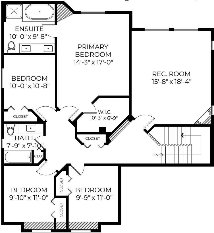
UPPER FLOOR PLAN Ceiling Height: 8'-0"
