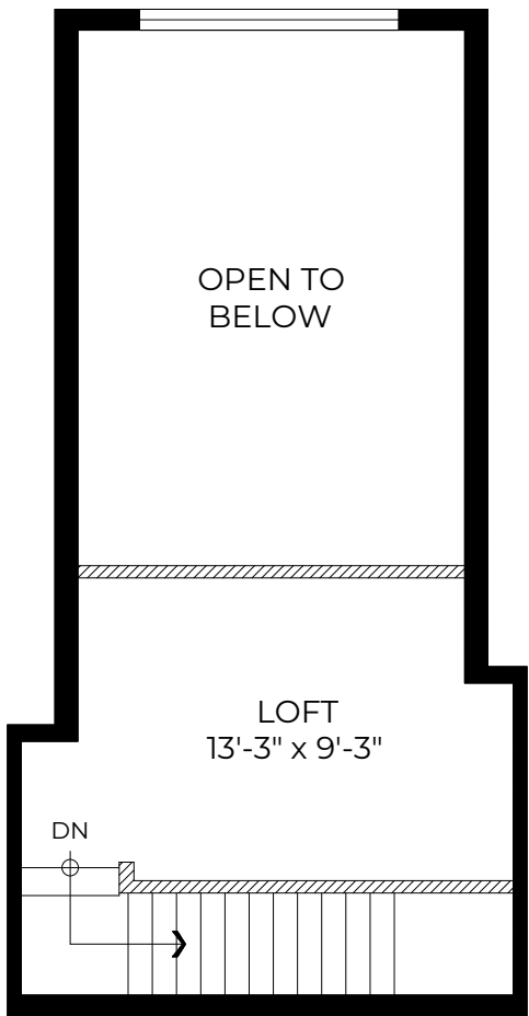
UPPER FLOOR PLAN Ceiling Height: 8'-0"
