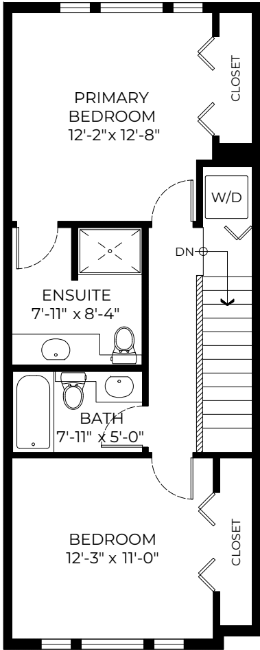
UPPER FLOOR PLAN Ceiling Height: 8'-1"
