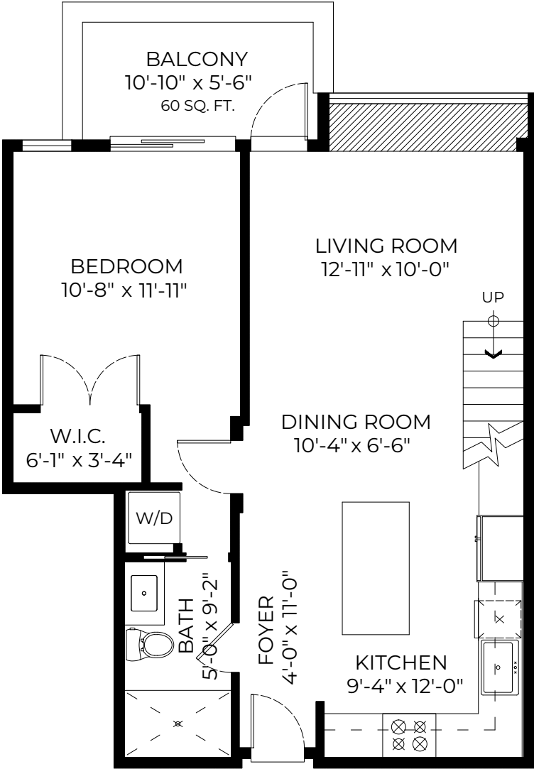
MAIN FLOOR PLAN Vaulted Ceiling Height: 13'-0"
