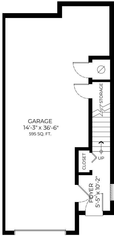
LOWER FLOOR PLAN Ceiling Height: 8'-0"
