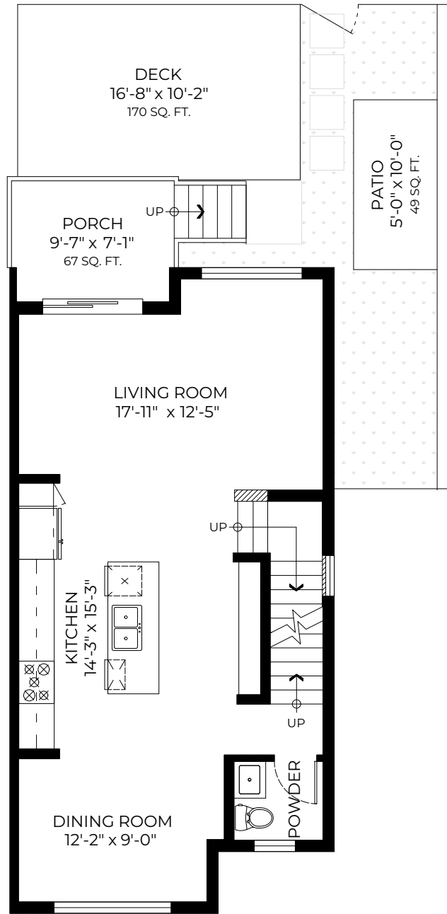
MAIN FLOOR PLAN Ceiling Height: 8'-0"
