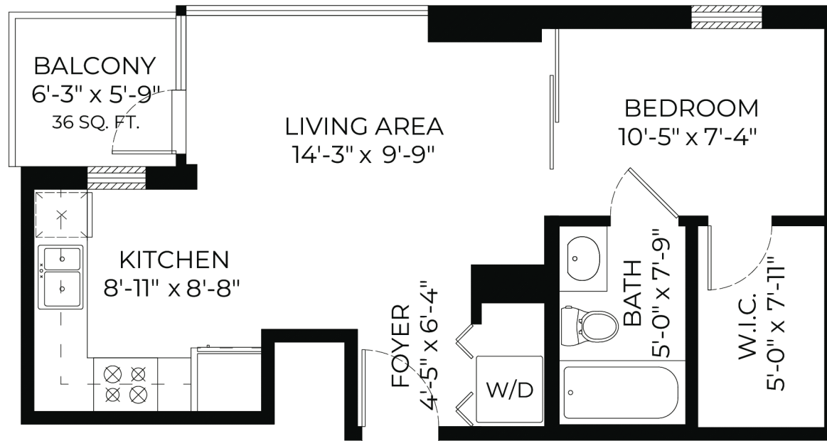
FLOOR PLAN Ceiling Height: 8'-0"
