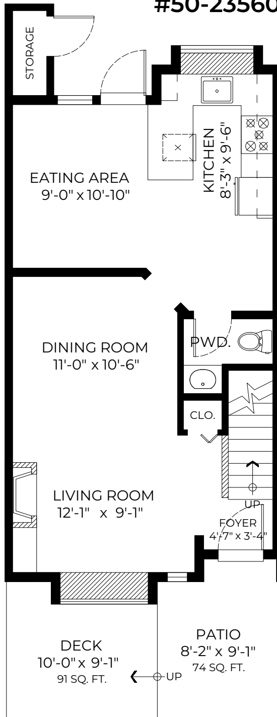
MAIN FLOOR PLAN Ceiling Height: 8'-0"
