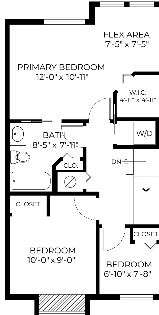
UPPER FLOOR PLAN Ceiling Height: 8'-0"
