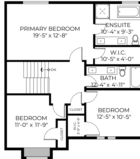
UPPER FLOOR PLAN Ceiling Height: 8'-0"
