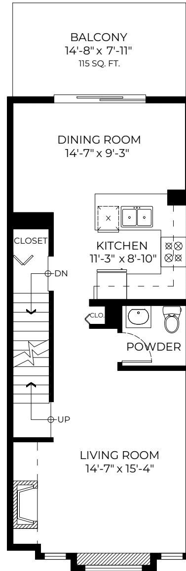
MAIN FLOOR PLAN Ceiling Height: 9'-0"
