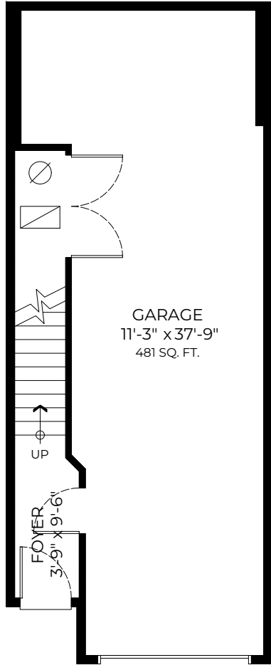
LOWER FLOOR PLAN Ceiling Height: 8'-0"
