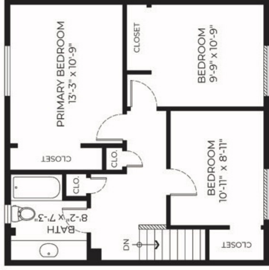
UPPER FLOOR PLAN Ceiling Height: 8'-0"
