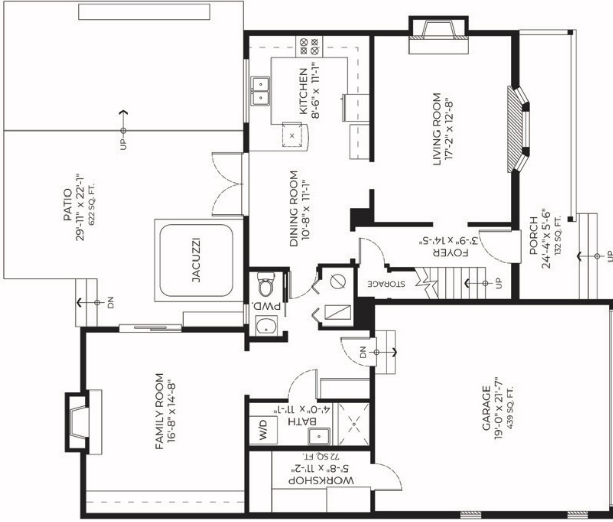
MAIN FLOOR PLAN Ceiling Height: 8'-0"
