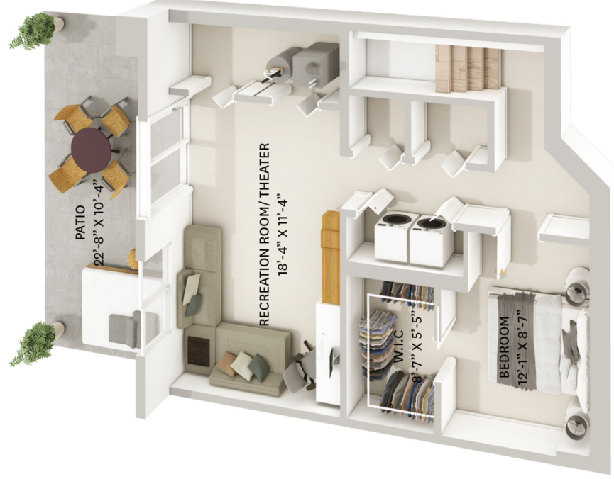
LOWER FLOOR PLAN Ceiling Height: 7'-6"
