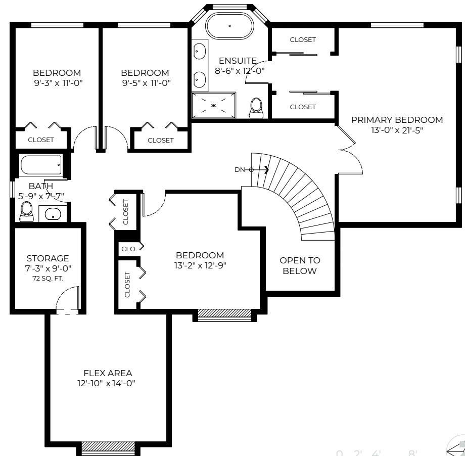
UPPER FLOOR PLAN Ceiling Height: 8'-0"
