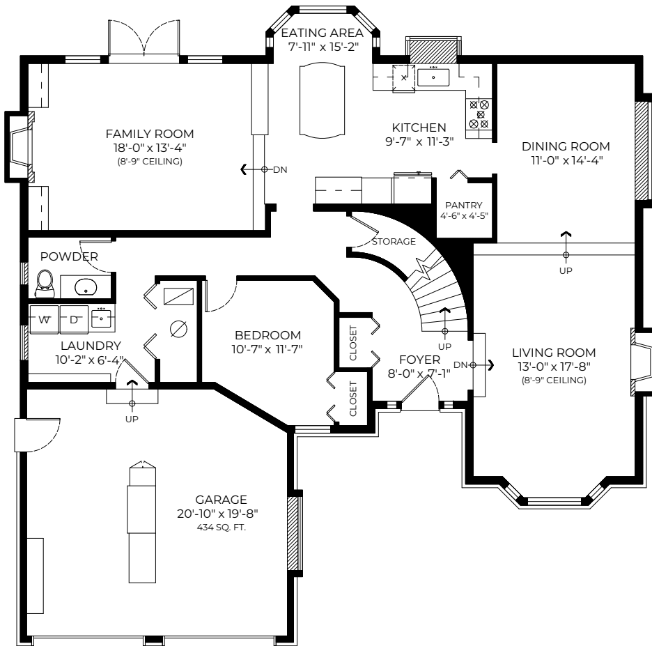
MAIN FLOOR PLAN Ceiling Height: 8'-0"
