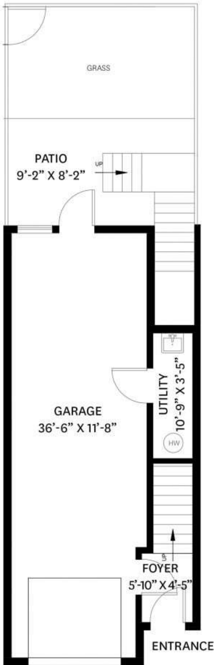
GARAGE AND LOWER FLOOR PLAN Ceiling Height: 8'-2"
