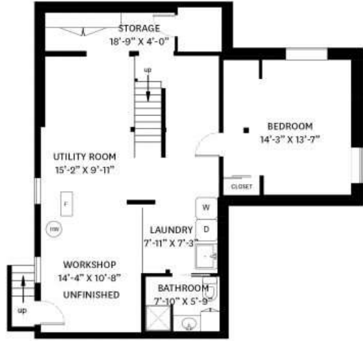
LOWER FLOOR PLAN Ceiling Height: 6'-5"
