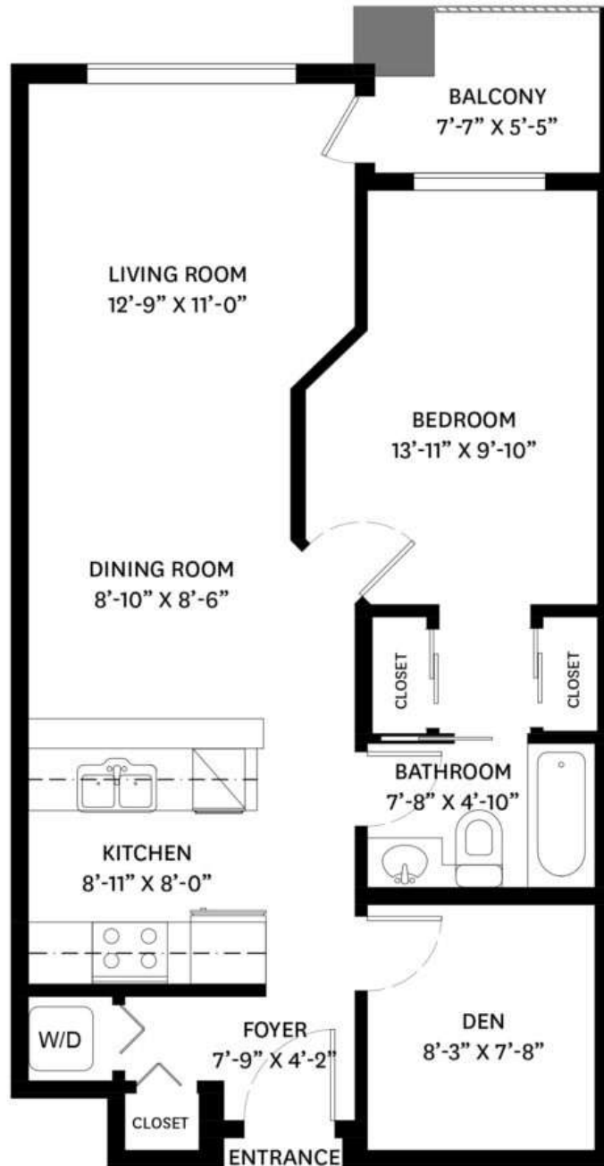
MAIN FLOOR PLAN Ceiling Height 7'-11"
