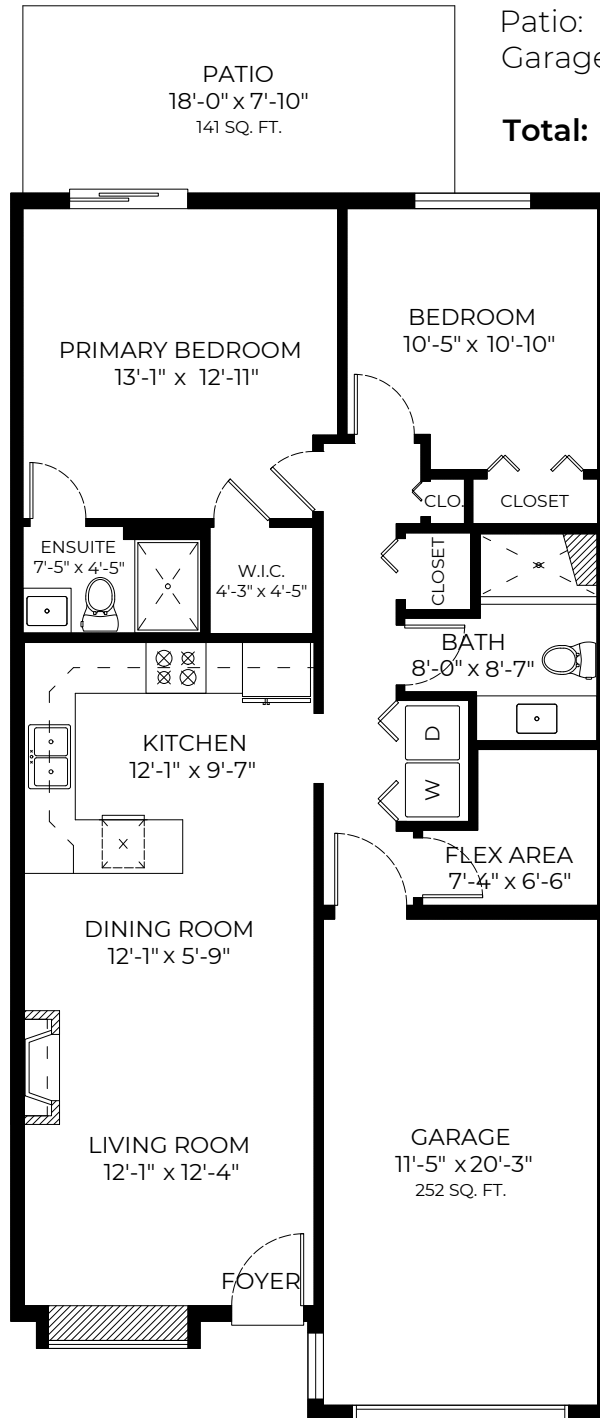
FLOOR PLAN Ceiling Height: 8'-0"
