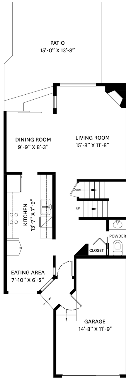
MAIN FLOOR PLAN Ceiling Height: 7'-11"
