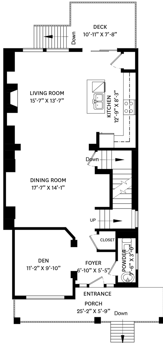
MAIN FLOOR PLAN Ceiling Height: 9'-0"
